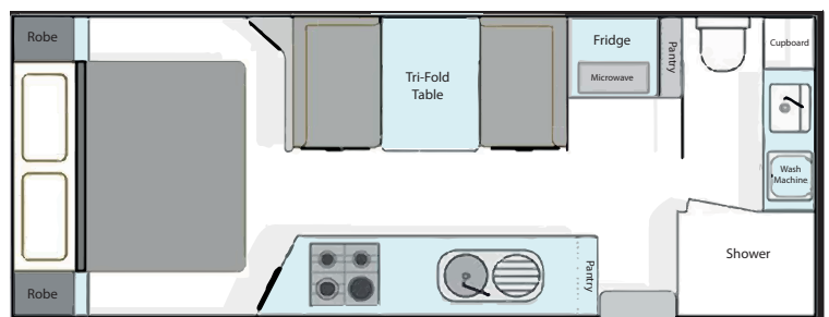
Floor plan. Illustration purpose only.
